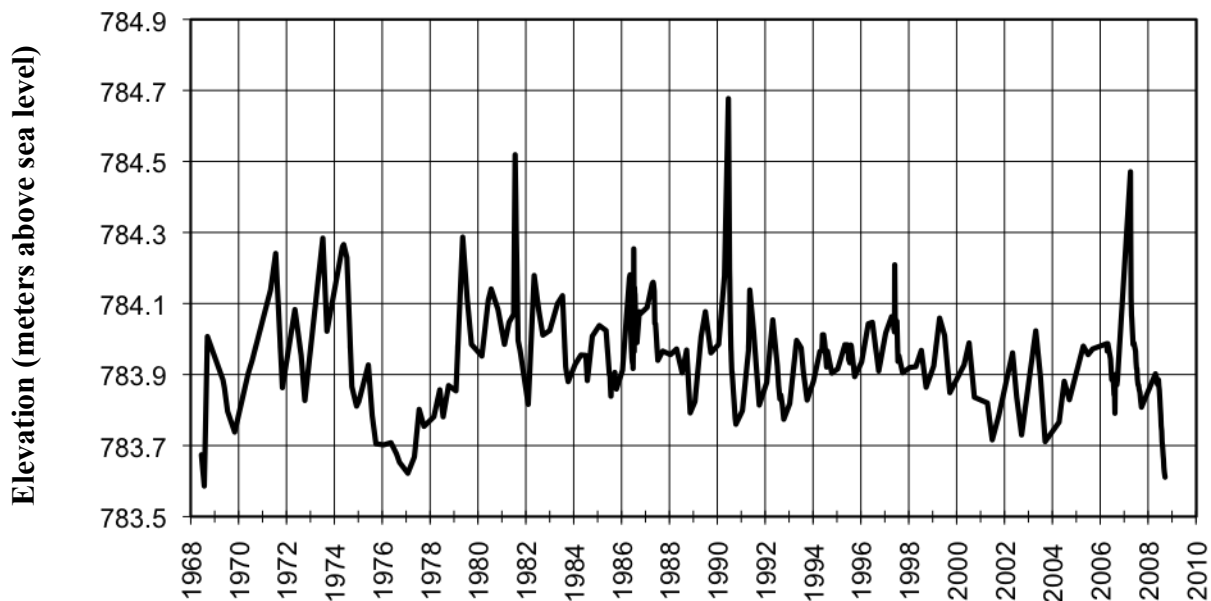
Figure 2. Historical water levels (meters above sea level (asl)) in Wizard Lake, Alberta 1968 – 2009.
