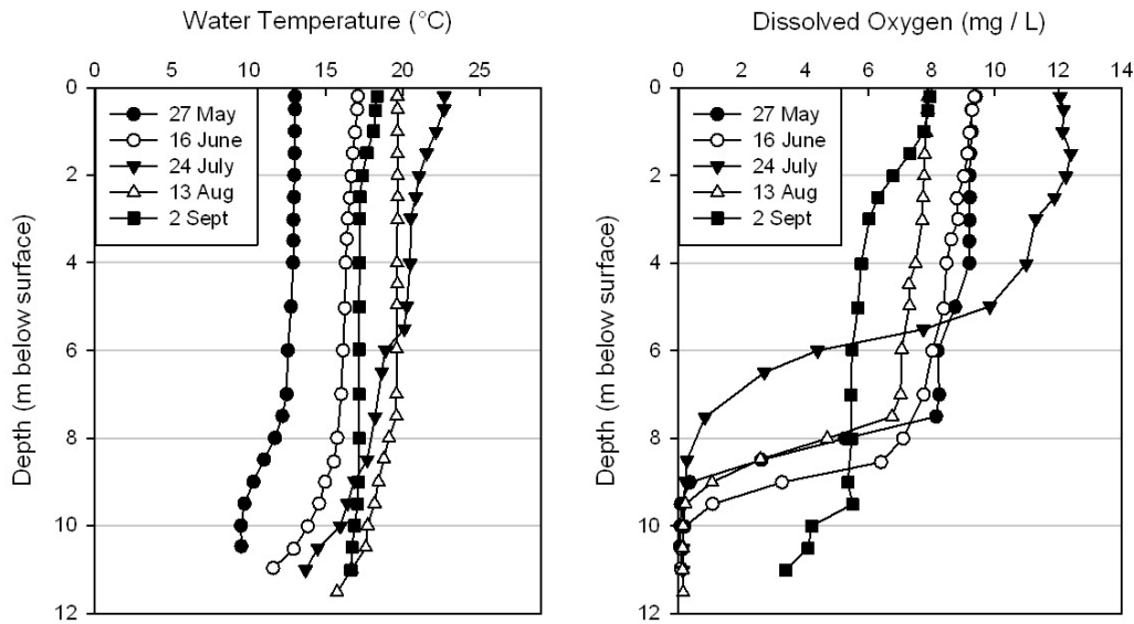
Figure 3. Water temperature (°C) and dissolved oxygen (mg/L) profiles for Wizard Lake during the summer of 2008.
